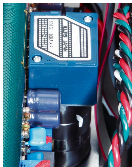
▲ Close to the inputs is the classic carbon-tracked ALPs volume potentiometer, which is moved by the stepper motor.
