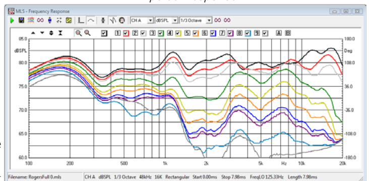
Frequency response
