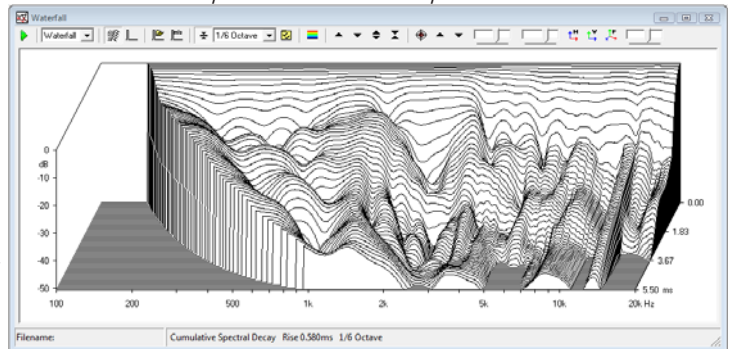
Waterfall
