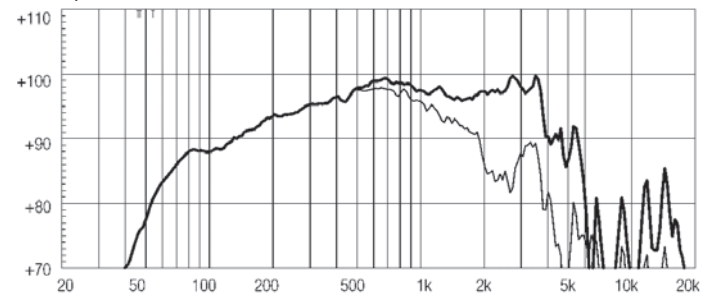
FREQUENCY RESPONSE CURVE OF 10MB600 MADE ON 30 LIT. ENCLOSURE TUNED AT 55HZ IN FREE FIELD (4P) ENVIRONMENT. ENCLOSURE CLOSES THE REAR OF THE DRIVER. THE THIN LINE REPRESENTS 45 DEG. OFF AXIS FREQUENCY RESPONSE
